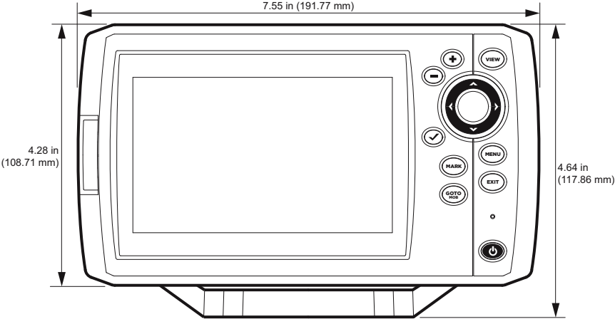
Gimbal Mount (HELIX 5)
