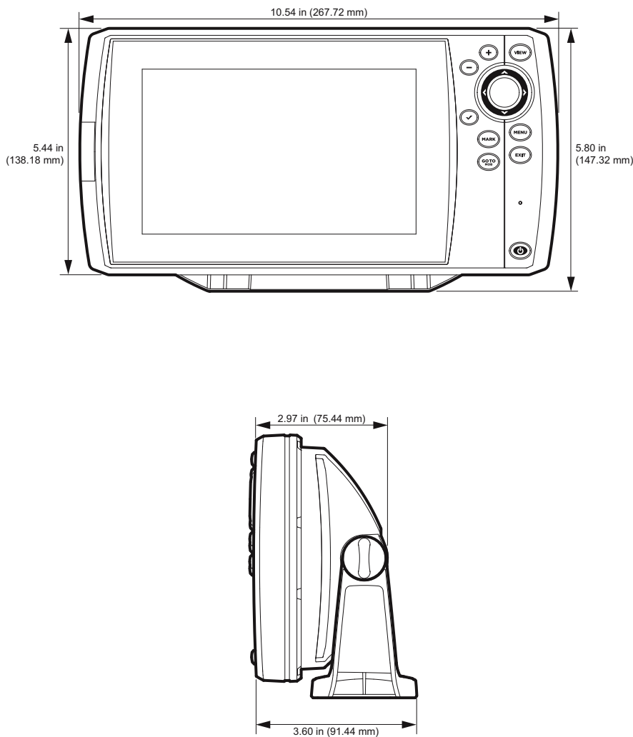
Gimbal Mount (HELIX 7)
